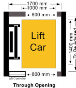
Through Opening
